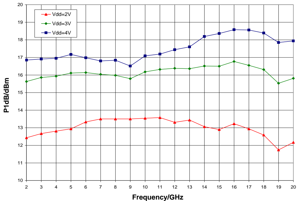
P1dB vs. V_{dd} , V_{gg} = 2.0\text{ V} , T_A = 25\text{ }^\circ\text{C}
