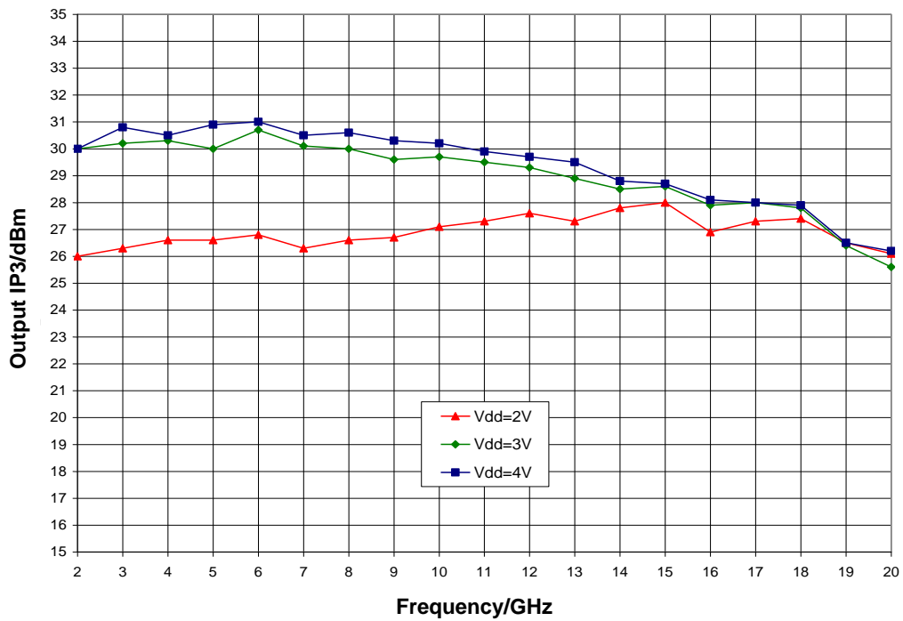
Output IP3 vs. V_{dd} , V_{gg} = 2.0\text{ V} , T_A = 25\text{ °C}
