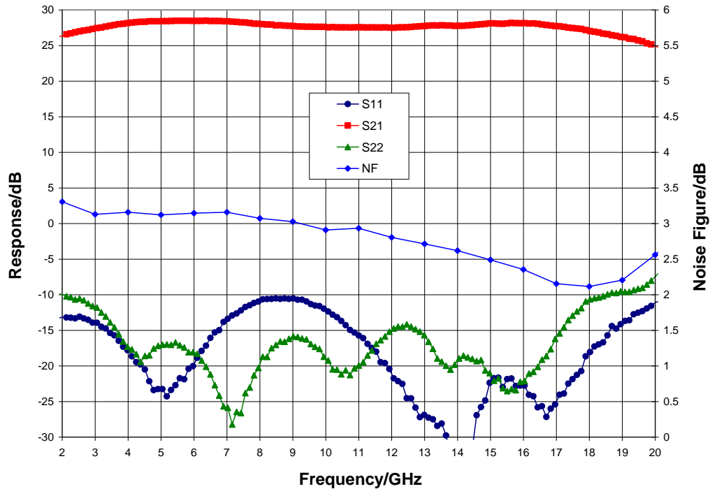
Narrow-band Performance, V_{dd} = 3.0\text{ V} , V_{gg} = 2.0\text{ V} , I_{dd} = 135\text{ mA} , T_A = 25\text{ }^\circ\text{C}
