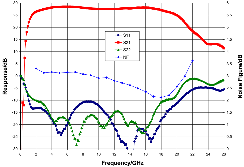
Broadband Performance, V_{dd} = 3.0\text{ V} , V_{gg} = 2.0\text{ V} , I_{dd} = 135\text{ mA} , T_A = 25\text{ }^\circ\text{C}
