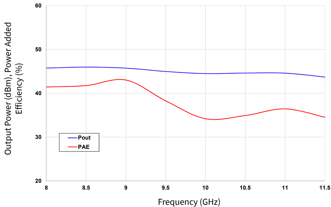
Figure 2. Output Power & Power Added Efficiency vs Frequency V_{DD} = 28\text{ V} , I_{DQ} = 0.8\text{ A} , P_{IN} = 27\text{ dBm} , Pulse Width = 100\mu\text{s} , 10% Duty Cycle, T_c = 85^\circ\text{C}
