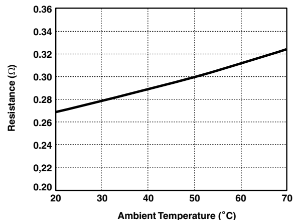
Figure 15. Switch Resistance vs Ambient Temperature
