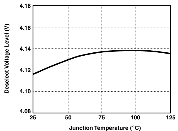
Figure 14. Deselect Threshold vs T_{JUNCT}
