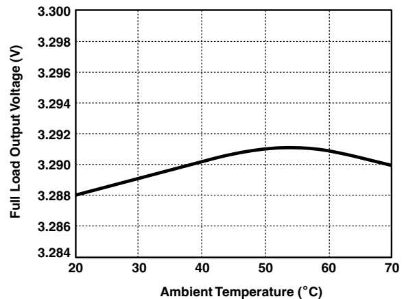
Figure 13. Regulator V_{OUT} vs T_{AMB} (250mA Load)
