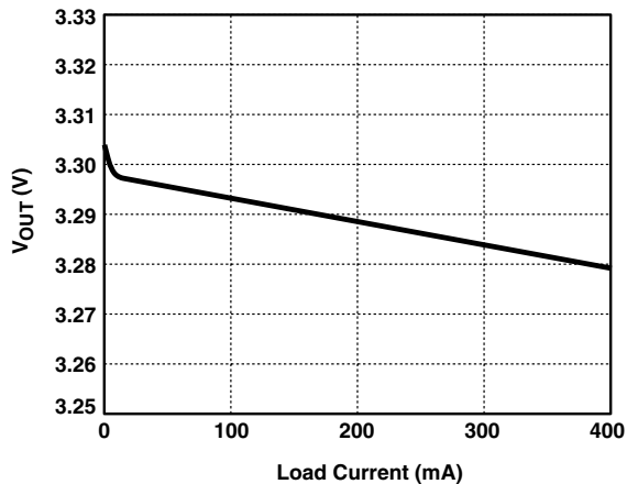
Figure 5. Load Regulation
