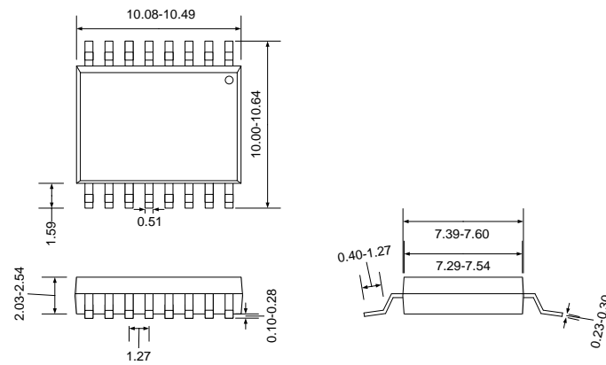
Drawing PSOIC16 (mm +/- 10%)
