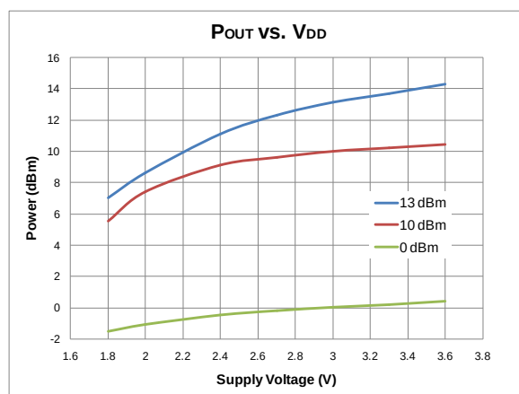
Figure 7. Output Power vs. Supply Voltages, F_{RF} = 433.92 MHz
