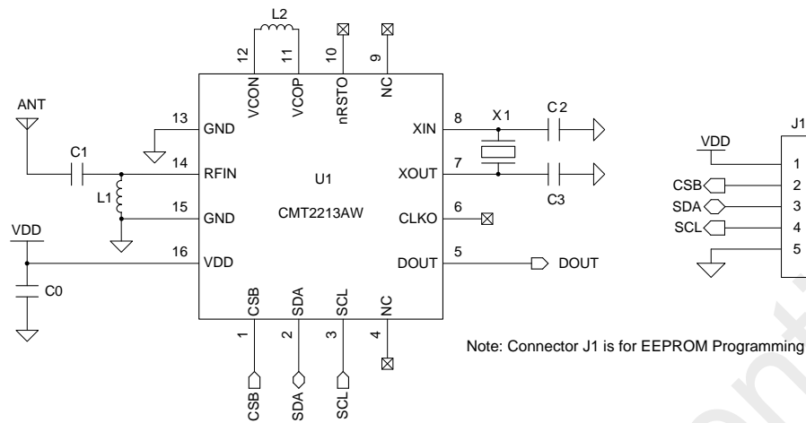
Figure 1. CMT2213AW Typical Application Schematic
