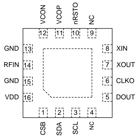
Figure 2. CMT2213AW Pin Assignments
