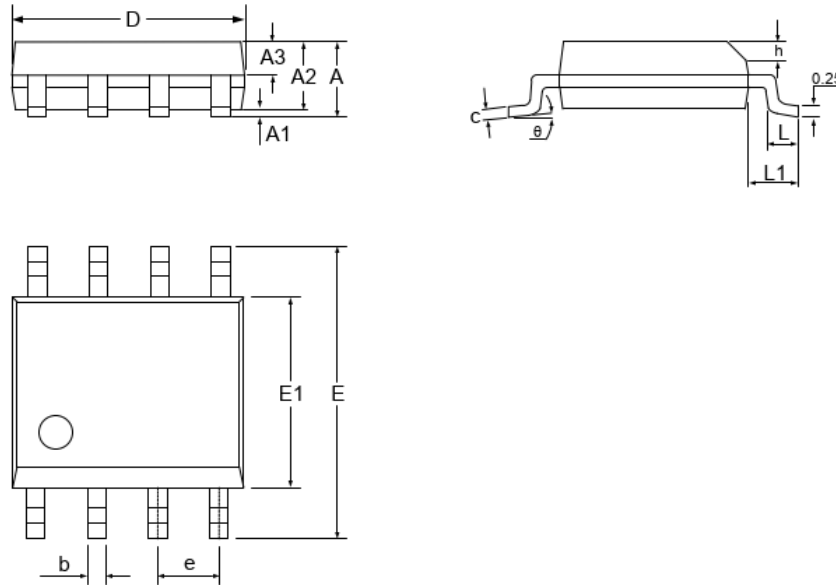
Figure 11. SOP8 Package
