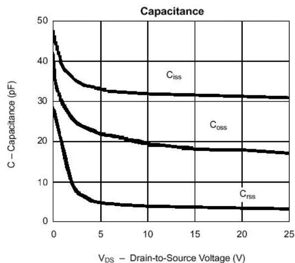
Figure 5. Capacitance
