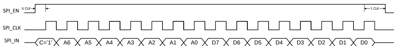
FIGURE 4: SPI WRITE TIMING
