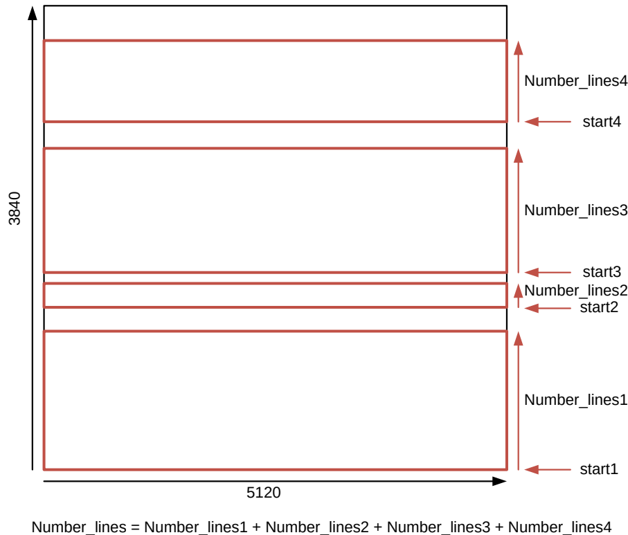
FIGURE 25: EXAMPLE OF 4 SUBWINDOWS READ-OUT
