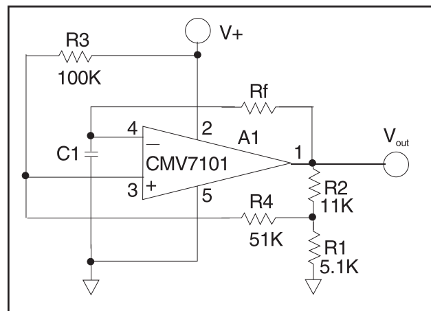
Figure 3. Single Rail Oscillator
