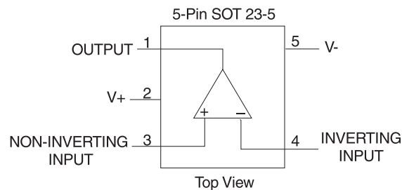
PIN DIAGRAM
