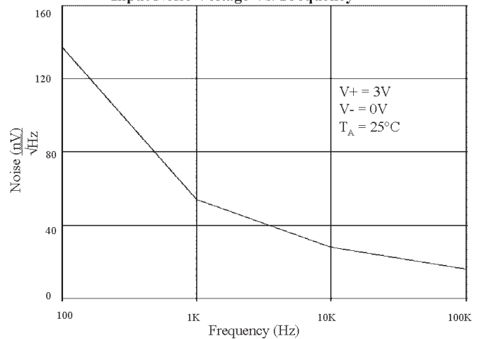
Input Noise Voltage Vs. Frequency
