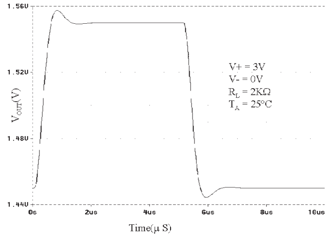
Inverting Small Signal Response
