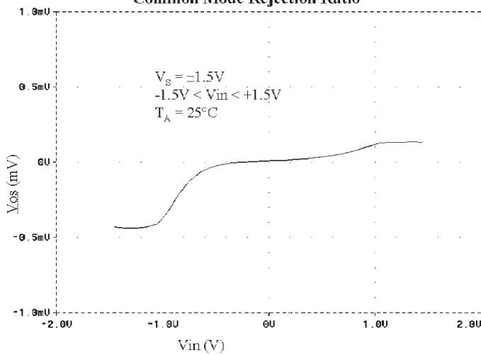
Common Mode Rejection Ratio
