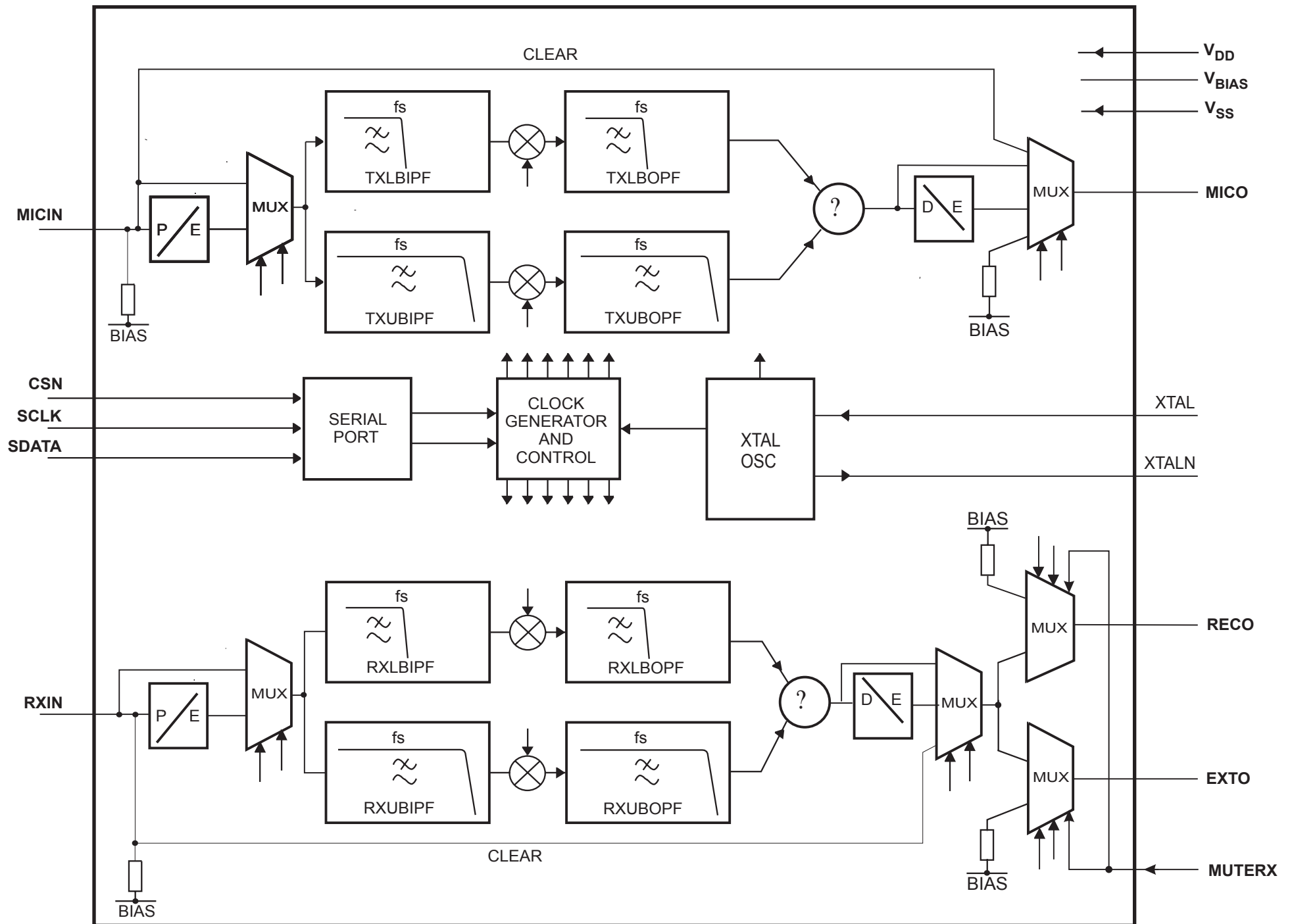
CMX264 Block Diagram
