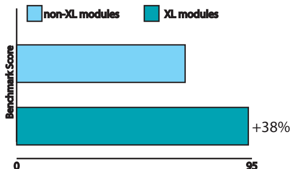
XL Performance Comparison (PCMark04 benchmark)
