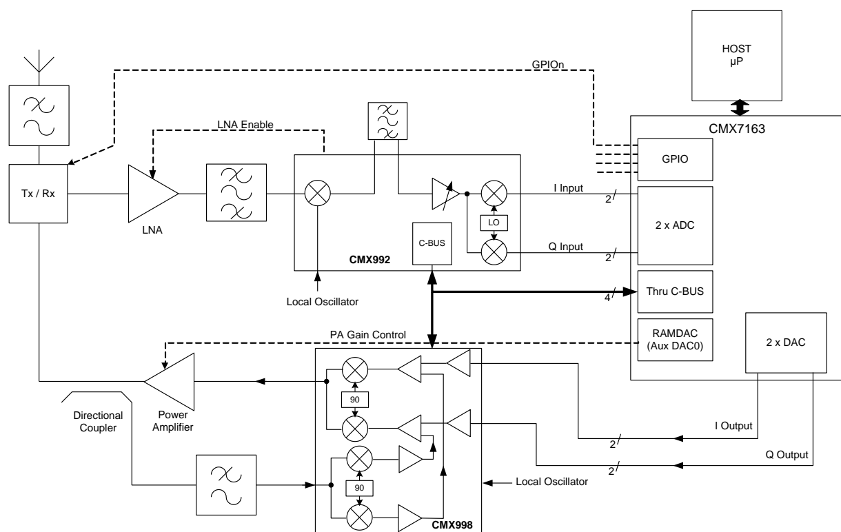
Figure 31 Outline Radio Design (I/Q in/out for QAM)
