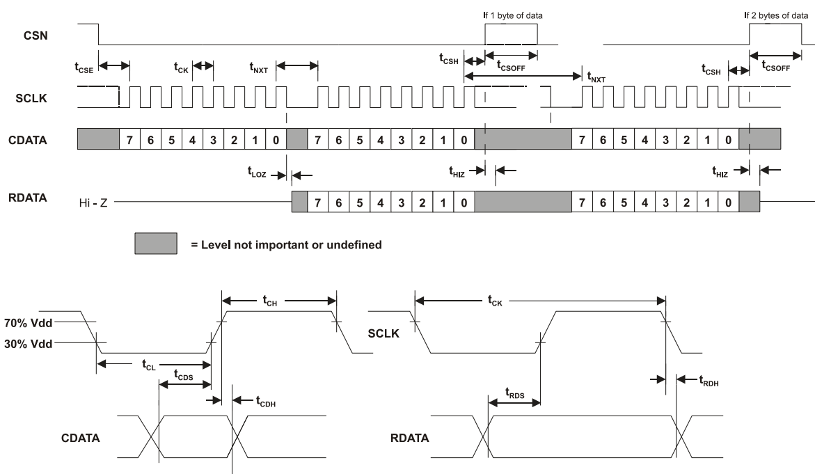
Figure 53 C-BUS Timing
