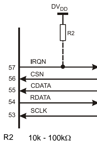
Figure 5 Recommended External Components – C-BUS Interface
