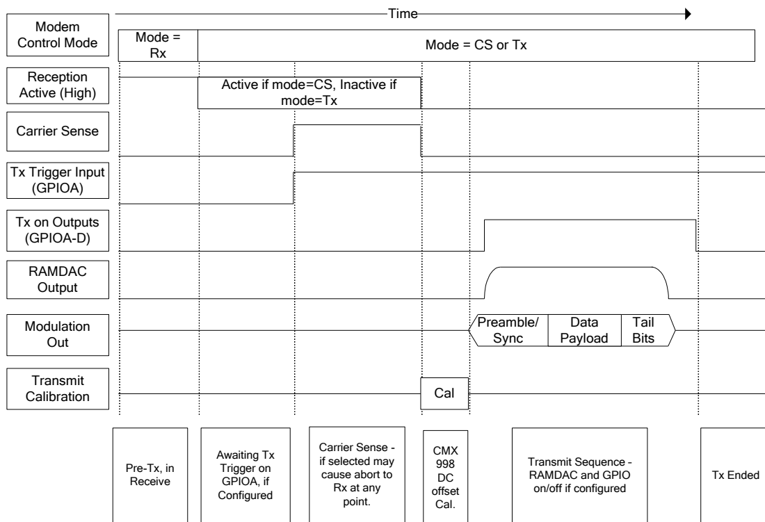
Figure 15 Transmit Sequence
