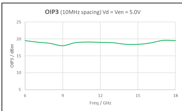
Figure 5: OIP3 (10MHz spacing) V_d = V_{en} = 5.0V
