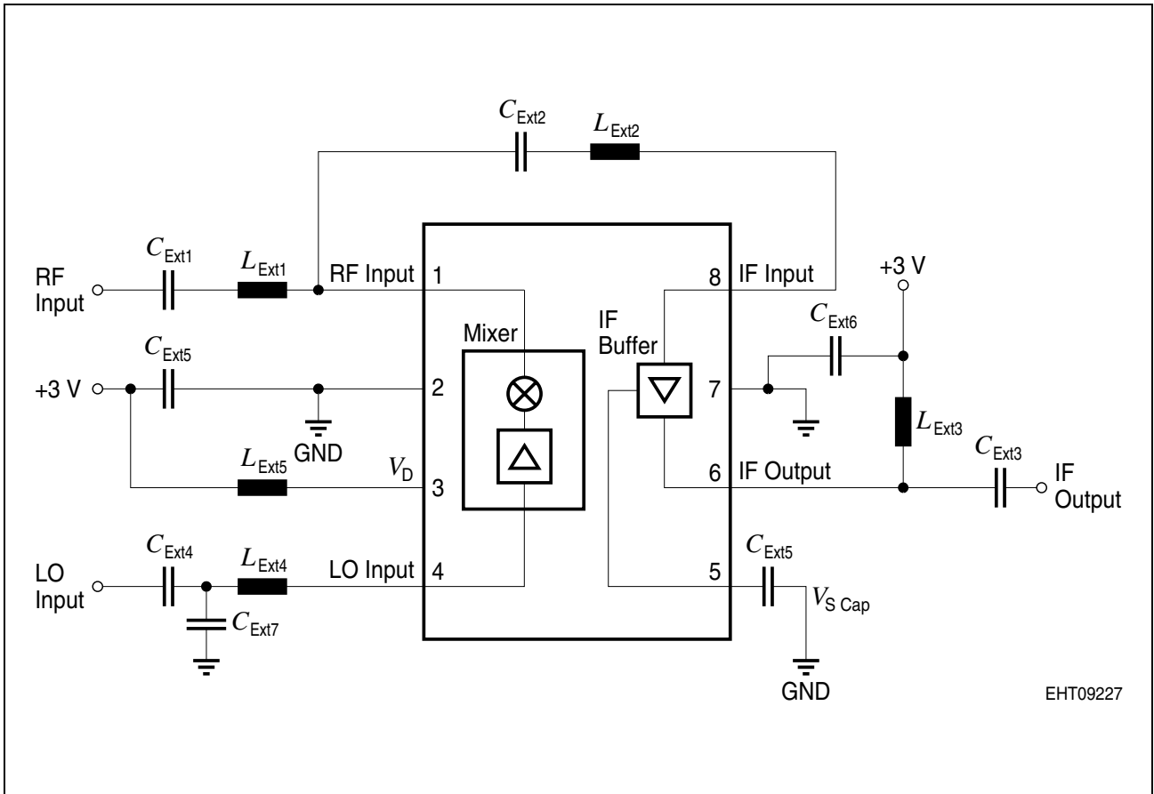
Figure 2 Test Circuit
