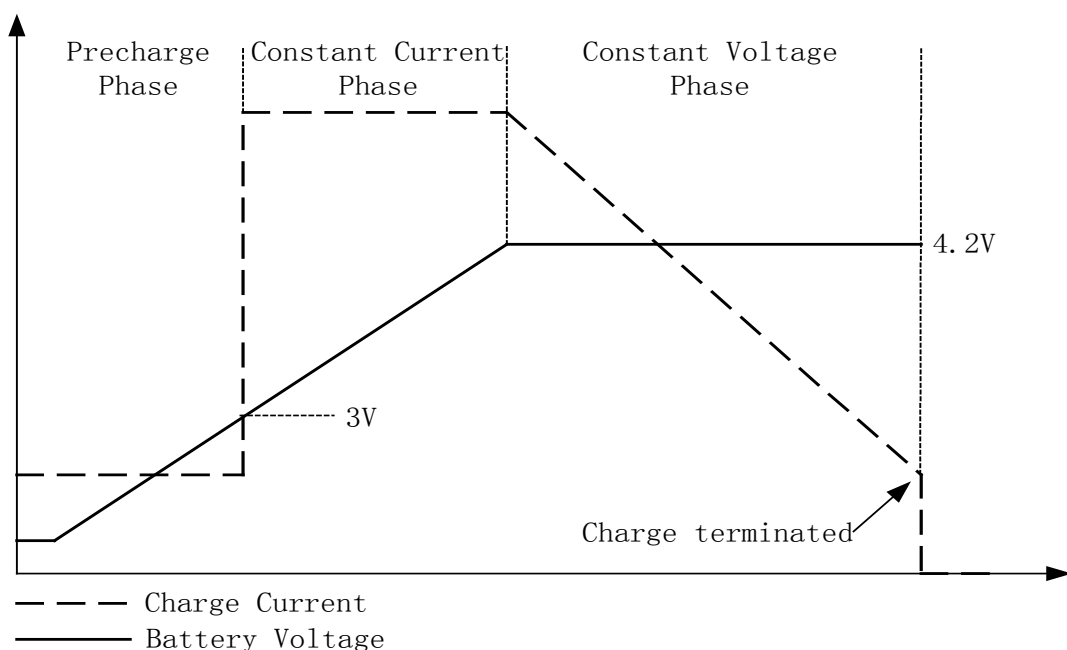
Figure 4 Charging Profile
