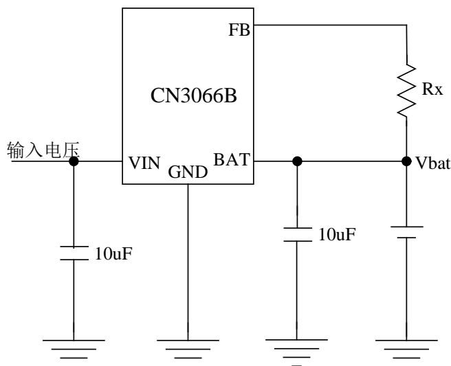
Figure 5 Adjusting Regulation Voltage in Constant Voltage Mode
