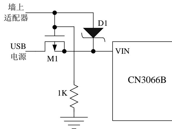
Figure 6 Combining Wall Adapter and USB Power
