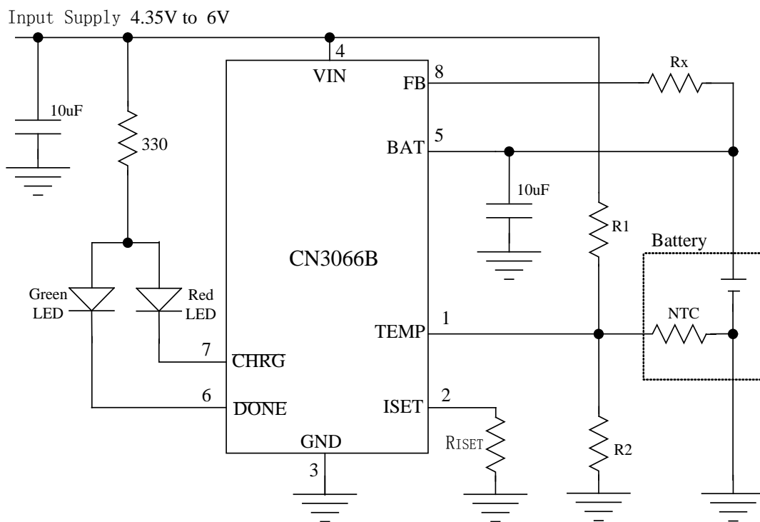
Figure 2 Application Circuit(Adjust Constant Voltage with R x )
