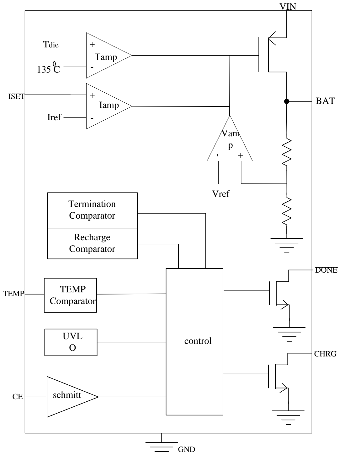
Figure 2 Block Diagram
