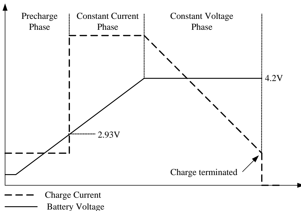
Figure 3 Charging Profile
