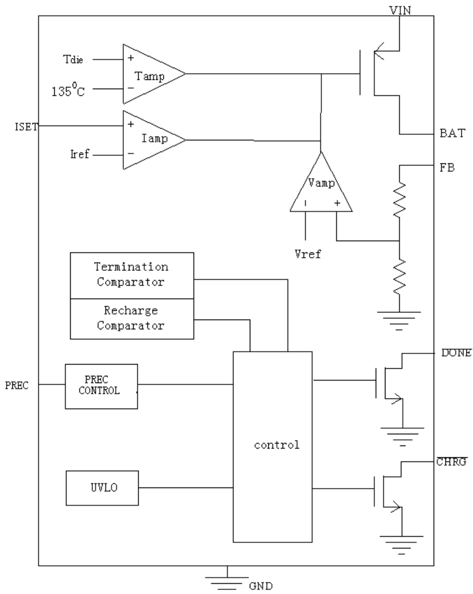
Figure 3 Block Diagram
