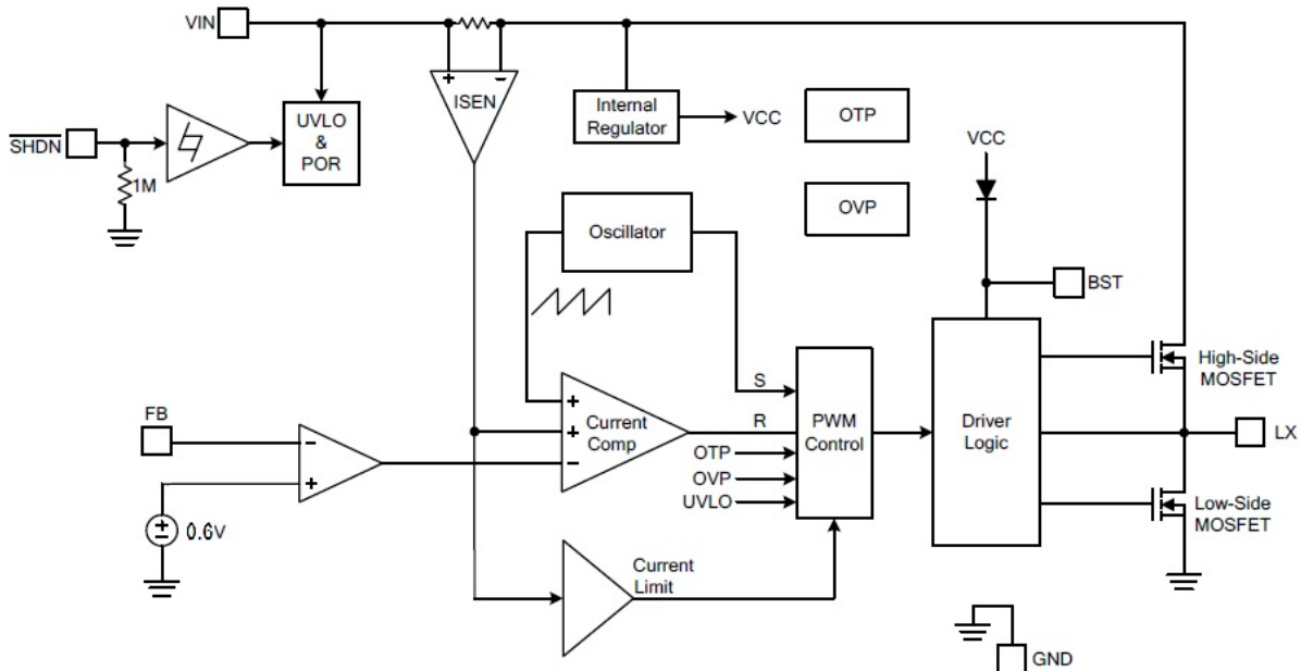
Block Diagram
