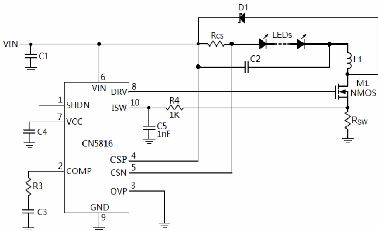
Figure 2 Typical Application Circuit of Buck Topology
