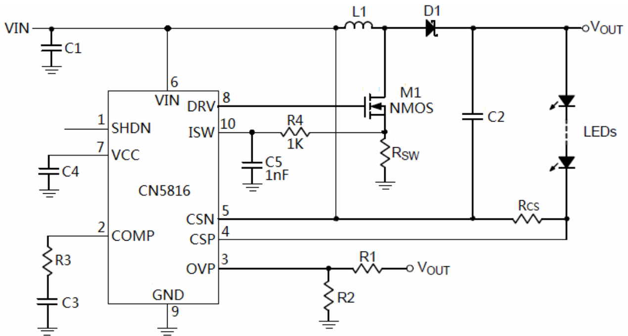
Figure 1 Typical Application Circuit of Buck-Boost Topology
