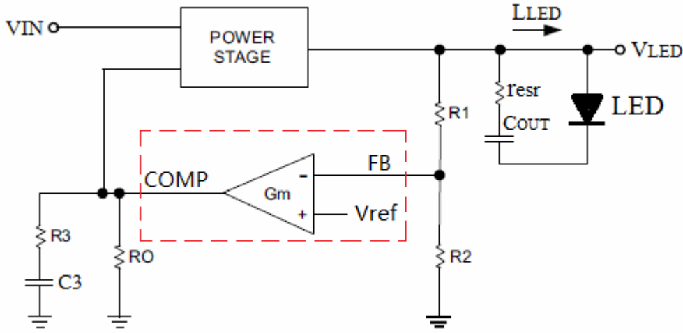
Figure 3 AC Response-Related Circuit
