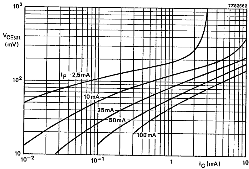
Fig. 14 T_{amb} = 25 ^{\circ}C ; typical values.
