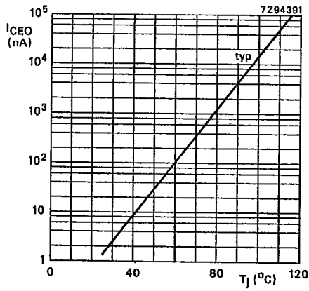
Fig. 12 V_{CE} = 10 V.
