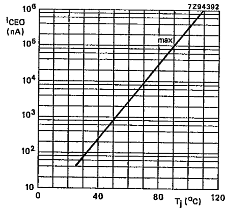
Fig. 13 V_{CE} = 10 V.
