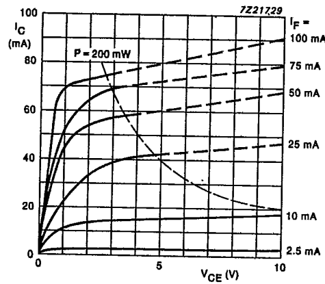
Fig.8 Typical values; T_{amb} = 25 ^{\circ}C .
