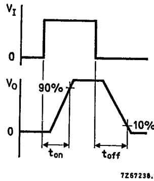
Fig.3 Waveforms.
