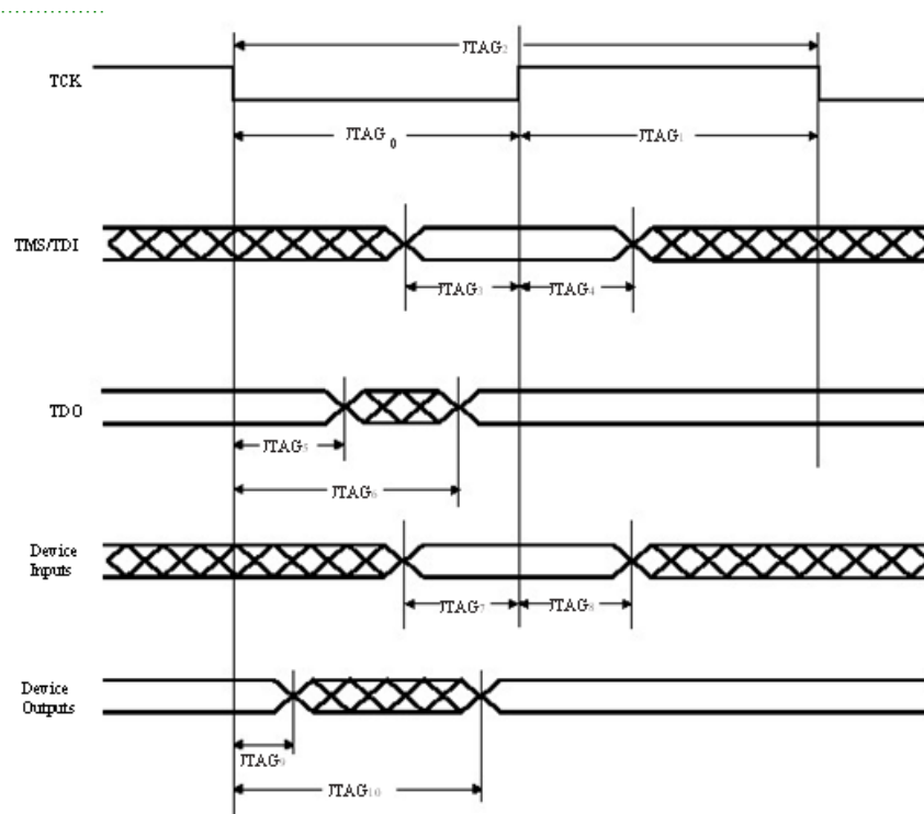
Figure 8-5: JTAG Timings
