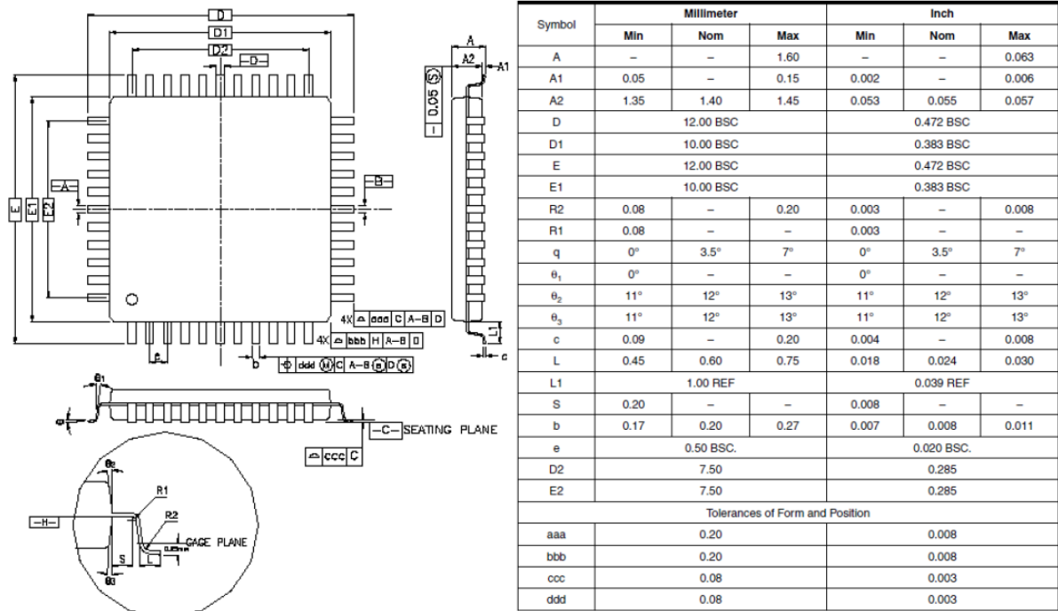
64-lead LQFP Package Drawing
