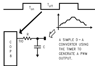
FIGURE 10. Timer Application
