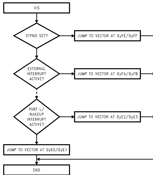
FIGURE 37. VIS Flowchart
