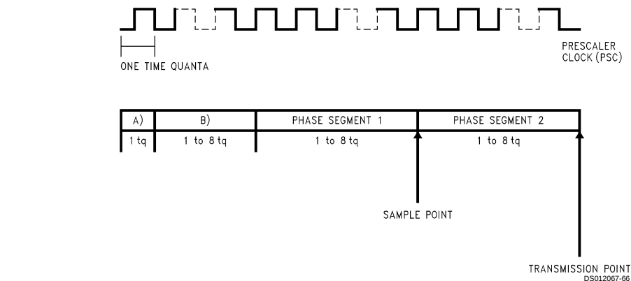
FIGURE 31. Bit Timing
