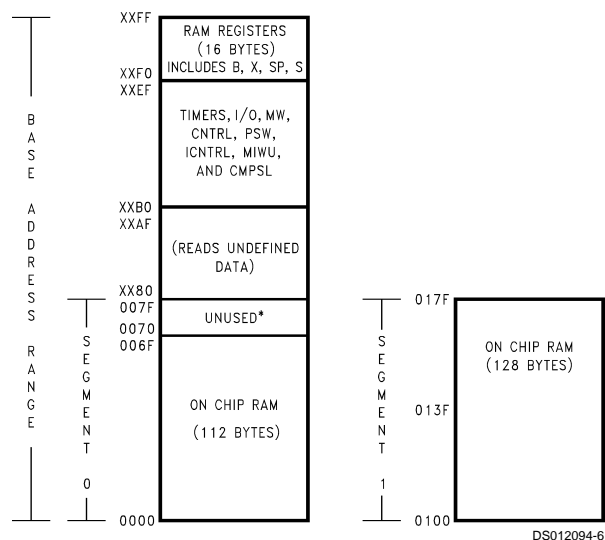
FIGURE 5. RAM Organization
