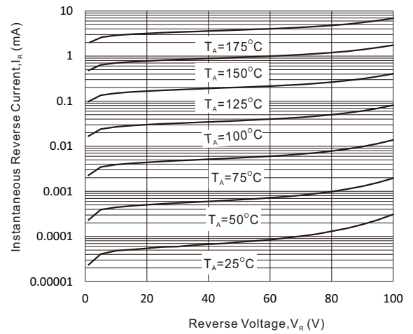
Fig. 2 - Reverse Characteristics
