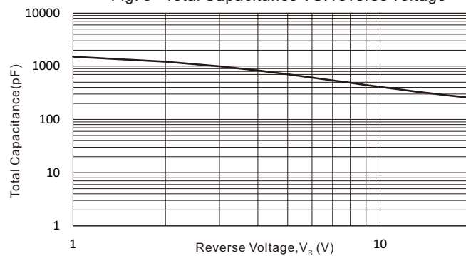
Fig. 5 - Total Capacitance VS. reverse voltage
