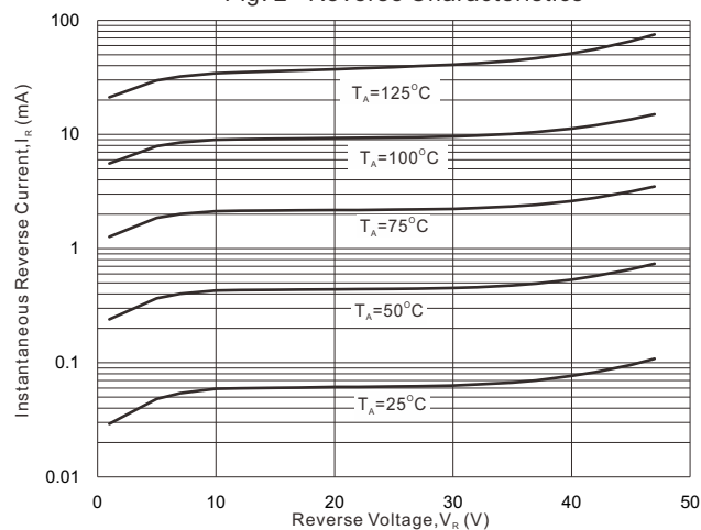
Fig. 2 - Reverse Characteristics
