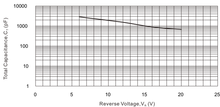
Fig. 5 - Total Capacitance VS. Reverse Voltage
