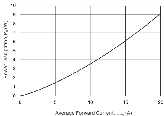
Fig. 3 - Forward Power Dissipation
