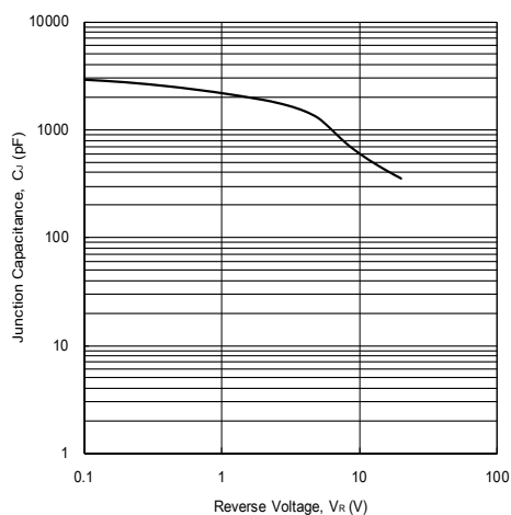
Fig. 5 - Junction Capacitance
