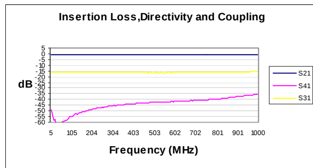
Typical Test Data – Insertion Loss, Coupling, Directivity
