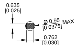
Pin Cross Section
