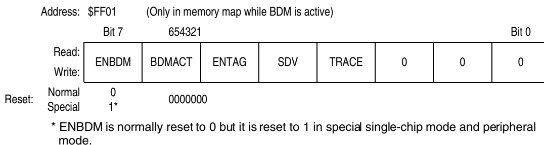
Figure 8-4. BDM Status Register (STATUS)
