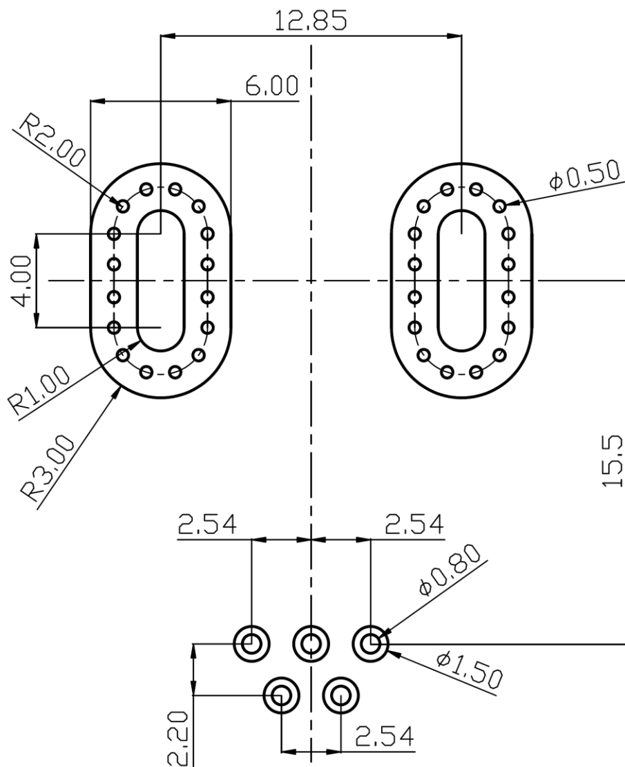
Figure 11. Package outline
