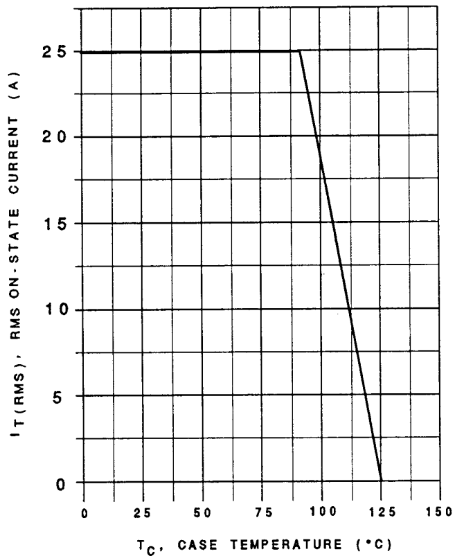
www.DataSheet4U.com RMS ON-STATE CURRENT vs. CASE TEMPERATURE
