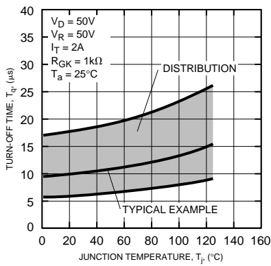
TURN-OFF TIME VS. JUNCTION TEMPERATURE (TYPICAL)
