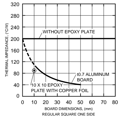
THERMAL IMPEDANCE VS. BOARD DIMENSIONS
