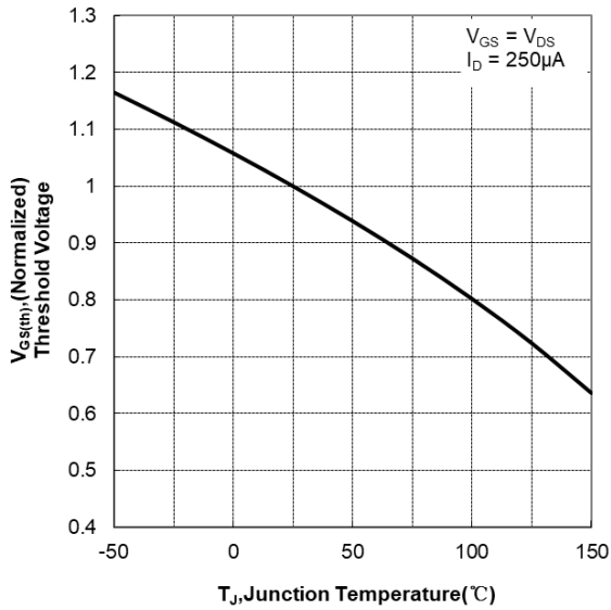
Figure.10 Typical Theshold Voltage vs Junction Temperatu
