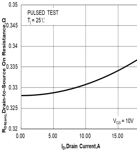
Figure.8 Typical Drain to Source ON Resistance vs Drain Current
