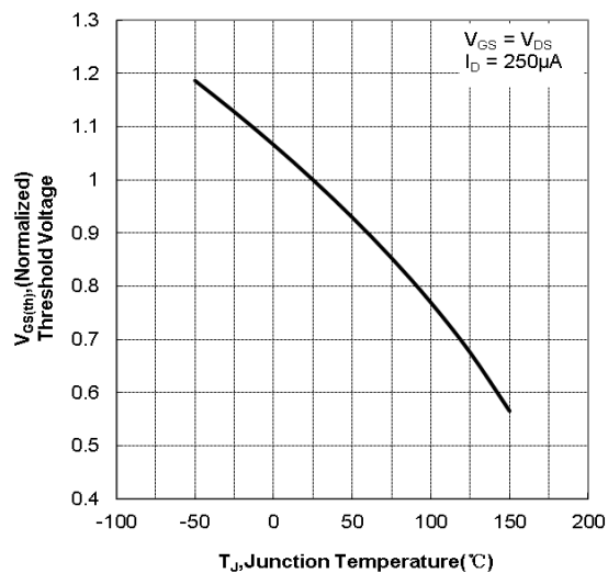
Figure.10 Typical Theshold Voltage vs Junction Temperatuu
