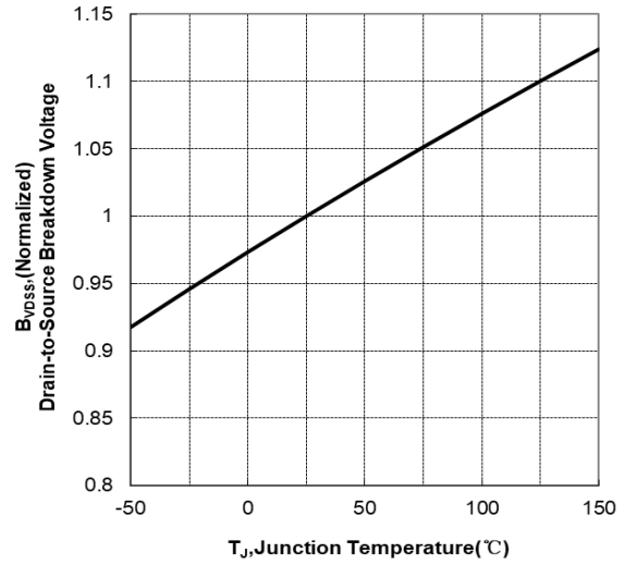
Figure 11 Typical Breakdown Voltage vs Junction Temperature
