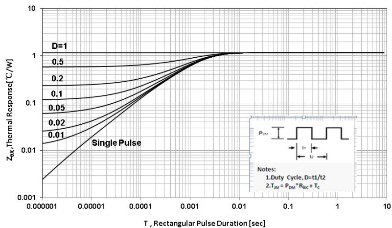
Figure.5 Maximum Effective Thermal Impedance , Junction to Case
