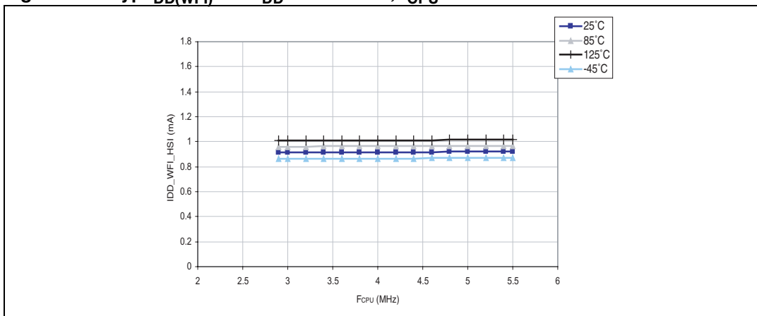
Figure 14. Typ I_{DD(WFI)} vs. V_{DD} HSI RC osc, f_{CPU} = 16 MHz
