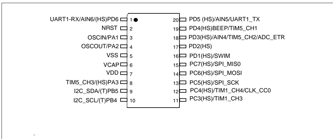
Figure 7 CR8F6123 SOP 20
