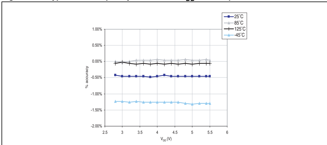
Figure 18. Typical HSI frequency variation vs V DD @ 4 temperatures
