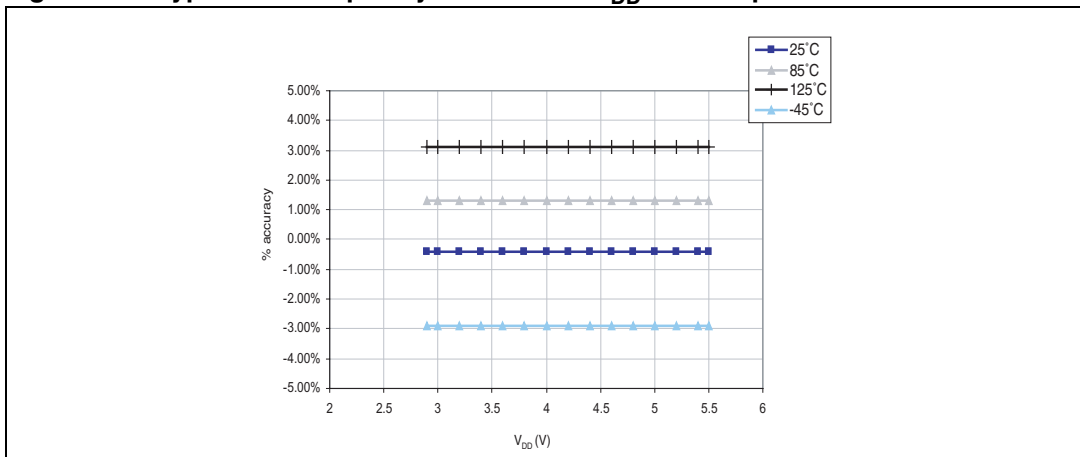
Figure 19. Typical LSI frequency variation vs V DD @ 4 temperatures
