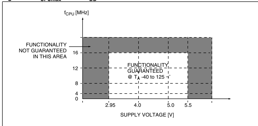
Figure 7. f CPUmax versus V DD
