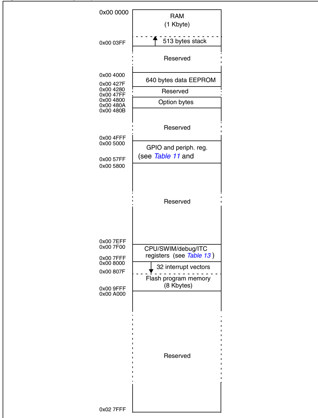
Figure 4. Memory map
