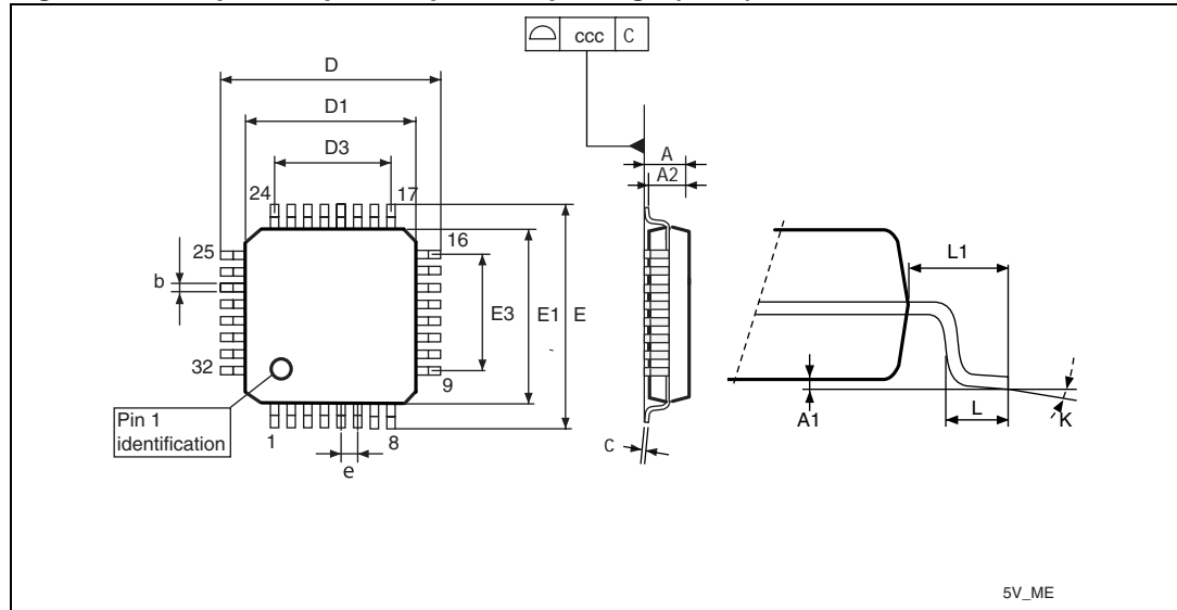
Figure 42. 32-pin low profile quad flat package (7 x 7)
