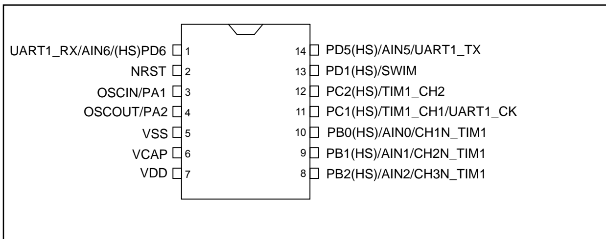
Figure6 CR8F6122B/M SOP/DIP 14
