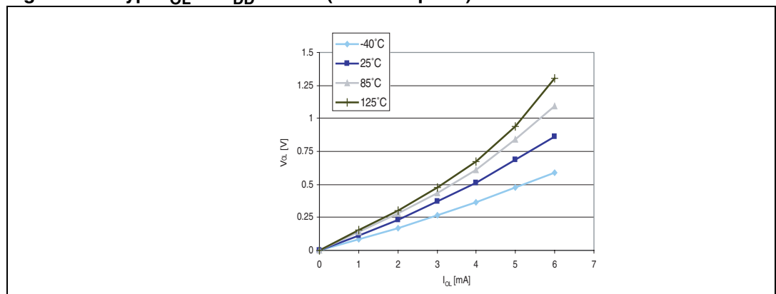
Figure 23. Typ. V OL @ V DD = 3.3 V (standard ports)
