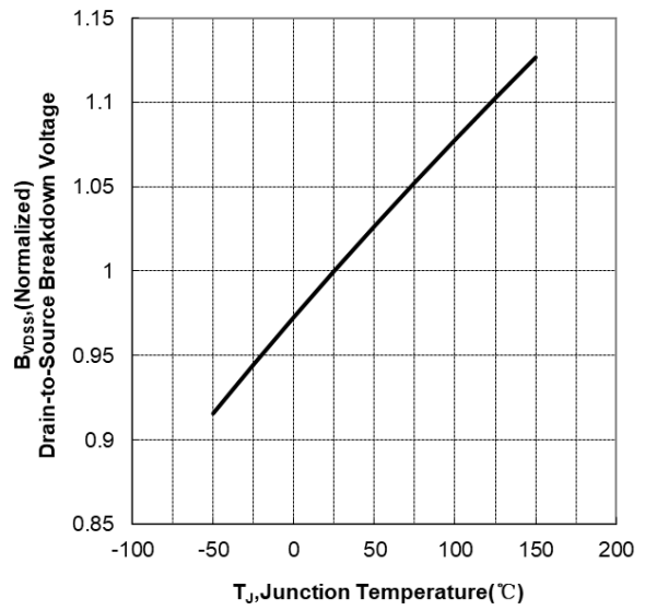
Figure.11 Typical Breakdown Voltage vs Junction
