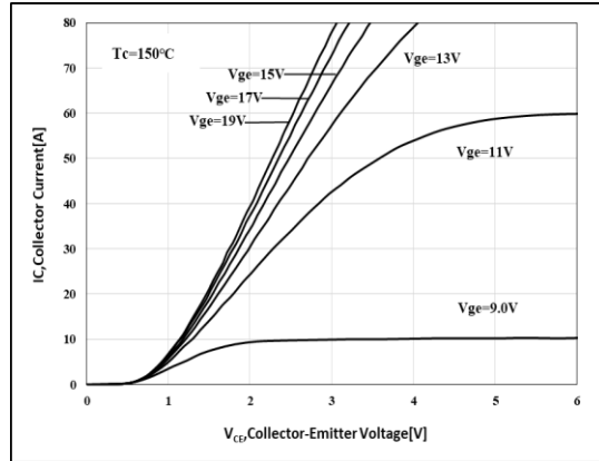
Figure 2. Output Characteristics
