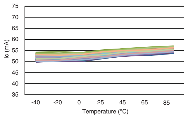
Figure 6.24 CRH02-400 Current Consumption over Temperature
