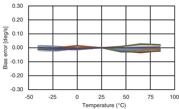
Figure 6.3 CRH02-200 Bias Variation over Temperature
