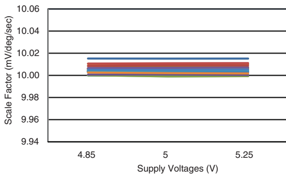
Figure 6.19 CRH02-200 Scale Factor Variation with Supply Voltage
