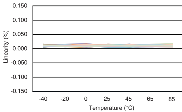
Figure 6.11 CRH02-200 Non-Linearity Error over Temperature
