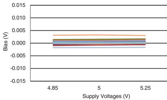
Figure 6.13 CRH02-025 Bias Variation with Supply Voltage
