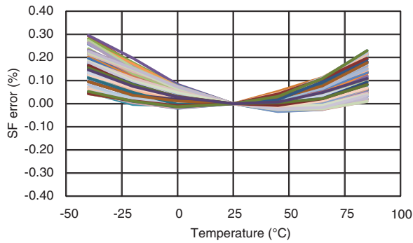
Figure 6.5 CRH02-025 Scale Factor Error over Temperature
