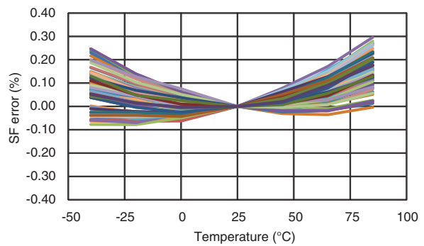
Figure 6.6 CRH02-100 Scale Factor Error over Temperature
