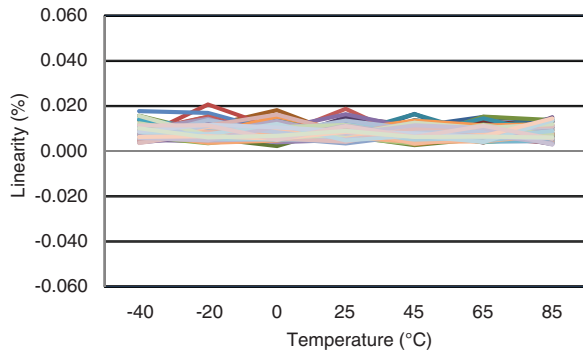
Figure 6.9 CRH02-025 Non-Linearity Error over Temperature
