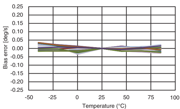
Figure 6.1 CRH02-025 Bias Variation over Temperature
