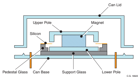
Figure 10.2 MEMS VSG3 Sensor
