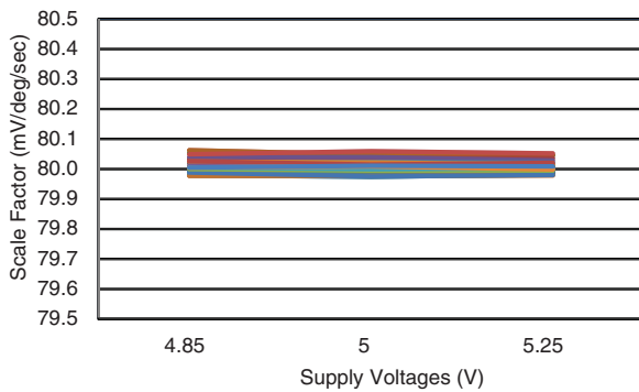
Figure 6.17 CRH02-025 Scale Factor Variation with Supply Voltage
