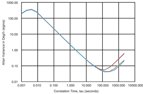
Figure 6.26 CRH02-025 Allan Variance
