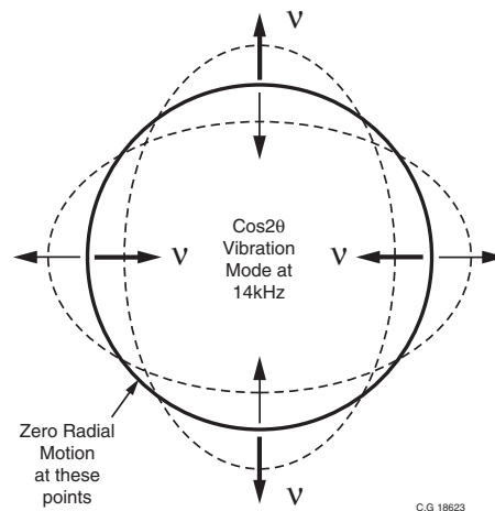
Figure 10.3 Primary Vibration Mode
