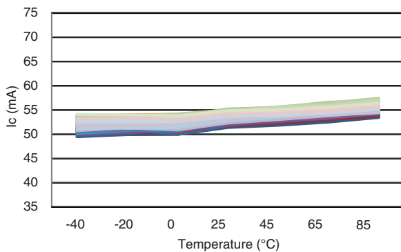
Figure 6.21 CRH02-025 Current Consumption over Temperature
