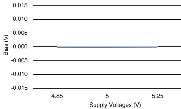
Figure 6.15 CRH02-200 Bias Variation with Supply Voltage
