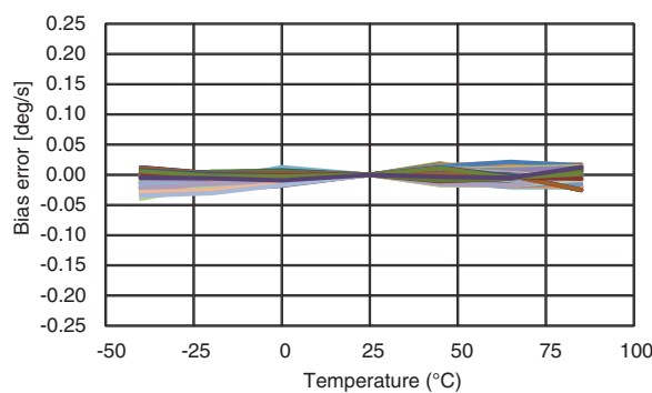
Figure 6.2 CRH02-100 Bias Variation over Temperature
