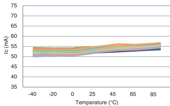
Figure 6.22 CRH02-100 Current Consumption over Temperature
