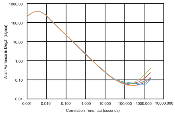
Figure 6.29 CRH02-400 Allan Variance
