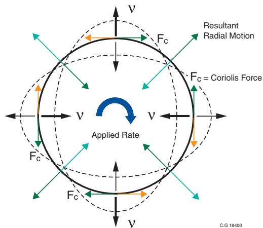
Figure 10.4 Secondary Vibration Mode
