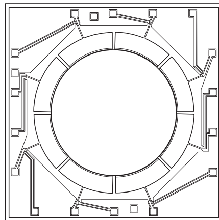
Figure 10.1 Silicon MEMS Ring
