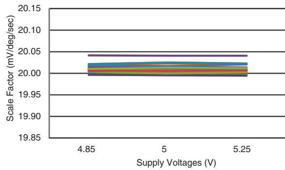
Figure 6.18 CRH02-100 Scale Factor Variation with Supply Voltage
