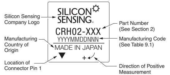
Figure 9.1 Part Marking
