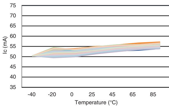
Figure 6.23 CRH02-200 Current Consumption over Temperature
