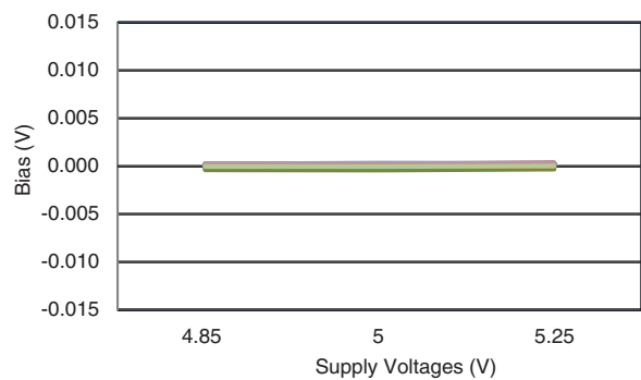
Figure 6.14 CRH02-100 Bias Variation with Supply Voltage
