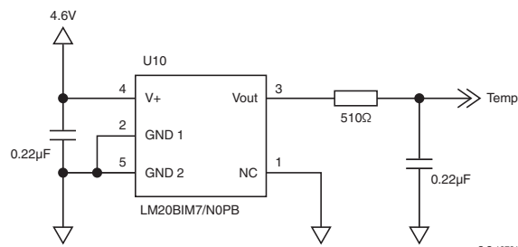
Figure 7.2 Temperature Sensor
