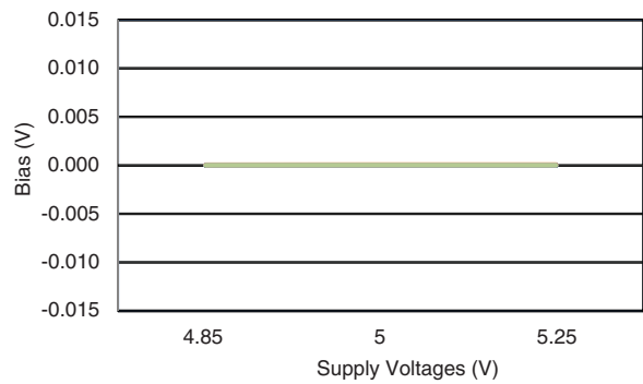
Figure 6.16 CRH02-400 Bias Variation with Supply Voltage
