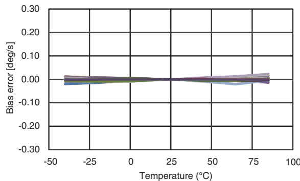
Figure 6.4 CRH02-400 Bias Variation over Temperature
