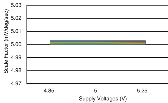
Figure 6.20 CRH02-400 Scale Factor Variation with Supply Voltage
