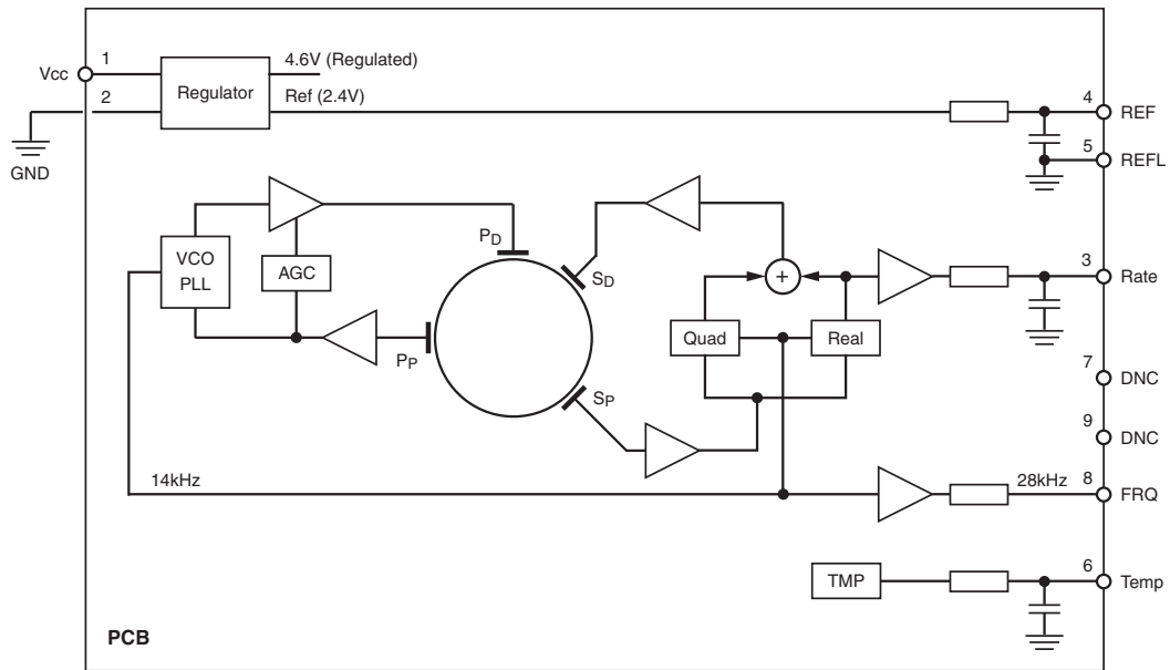
Figure 1.1 CRH02 Functional Block Diagram
