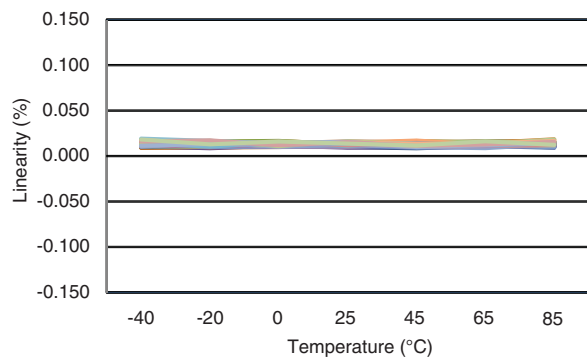
Figure 6.12 CRH02-400 Non-Linearity Error over Temperature
