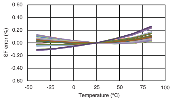
Figure 6.8 CRH02-400 Scale Factor Error over Temperature
