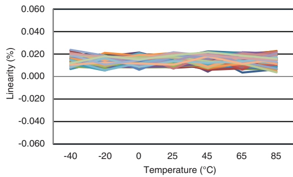
Figure 6.10 CRH02-100 Non-Linearity Error over Temperature
