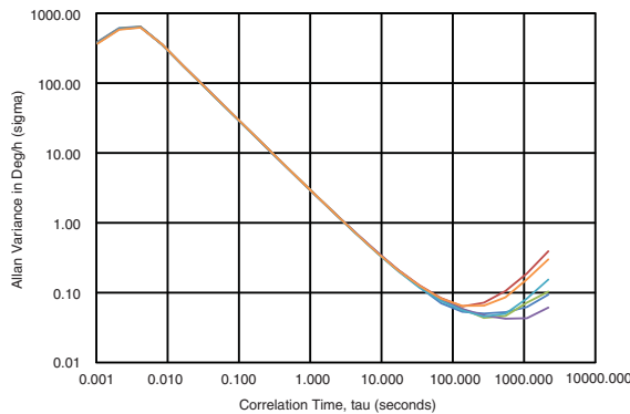
Figure 6.28 CRH02-200 Allan Variance
