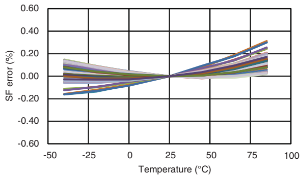
Figure 6.7 CRH02-200 Scale Factor Error over Temperature
