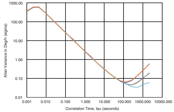
Figure 6.27 CRH02-100 Allan Variance
