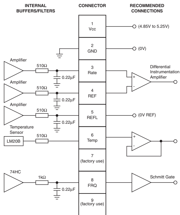
Figure 7.1 Typical Interface Schematic
