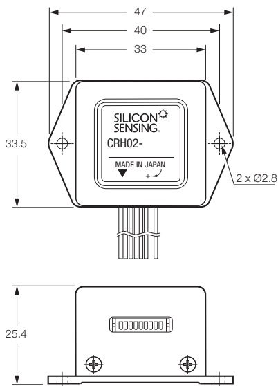
Figure 1.2 CRH02 Overall Dimensions
