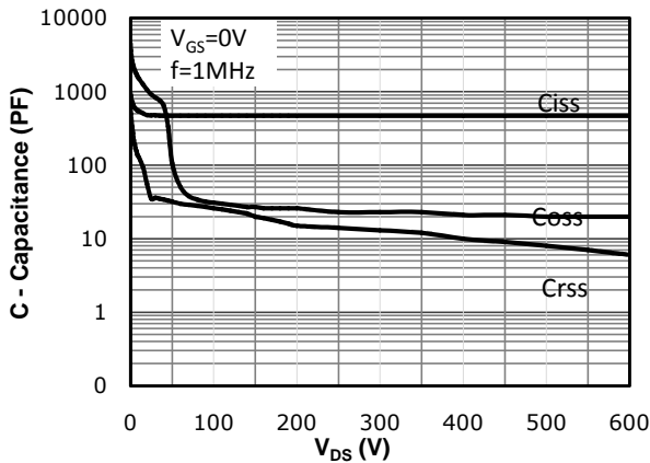
Fig 11: Capacitance Characteristics
