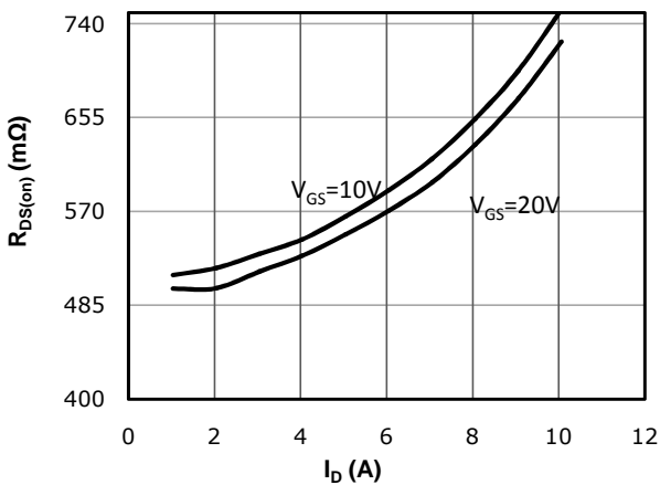
Fig 5: R DS(on) Vs I DS Characteristics (T C =25°C)
