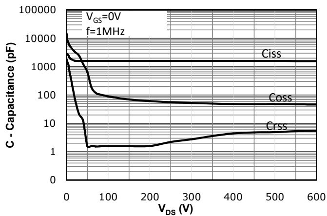
Fig 11: Capacitance Characteristics
