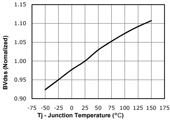
Fig 7: BVDSS vs. Temperature
