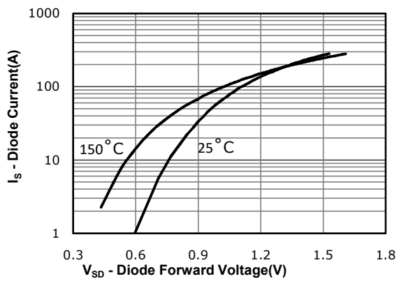
Fig 9: Body-diode Forward Characteristics
