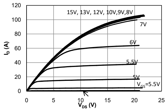
Fig 2. Output Characteristics (Tj=150°C)
