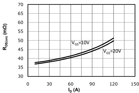
Fig 5: R ds(on) Vs Ids Characteristics(Tj=25°C)
