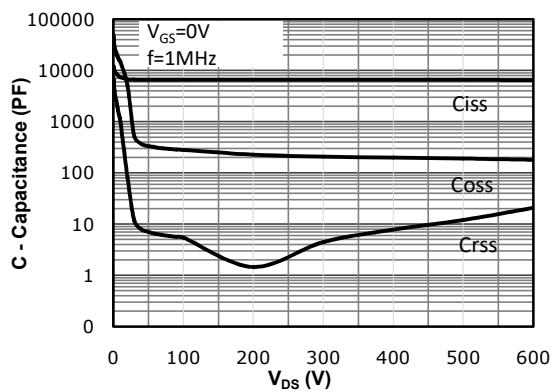
Fig 11: Capacitance Characteristics
