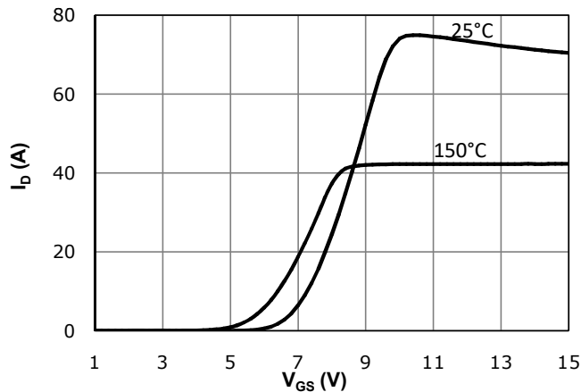
Fig 3: Transfer Characteristics
