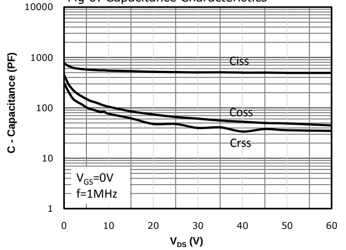
Fig 6: Capacitance Characteristics
