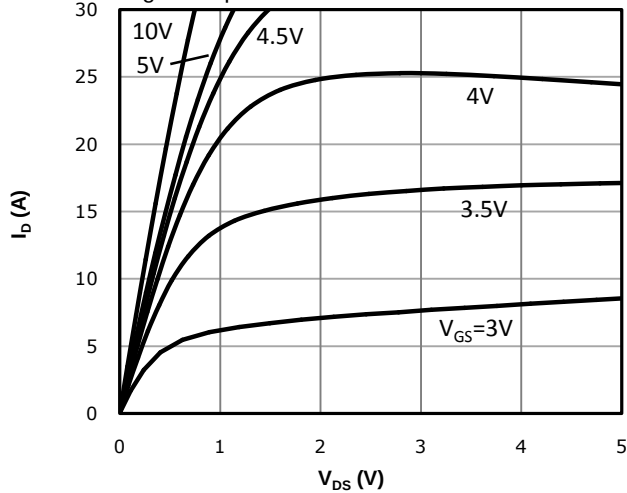
Fig 1: Output Characteristics
